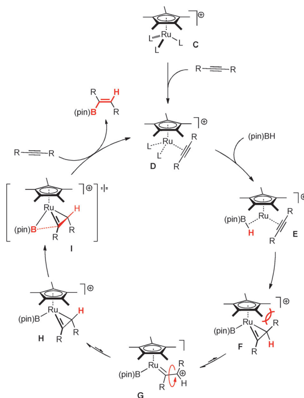
Scheme 4. Possible mechanism of the trans hydroboration.
